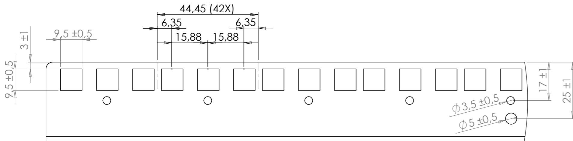
DETAIL A SCALE 1 : 1
